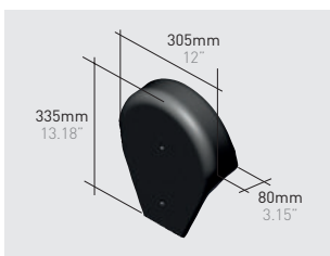
Q83*K | End cap round ridge klinker
