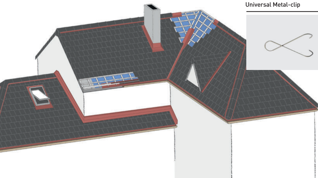
CAM26 Universal Metal-clip
